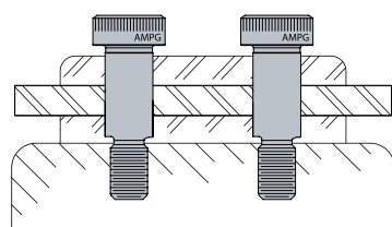
Shoulder Screw as a Guide
