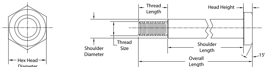
Dimensions and Tolerance Table — Inch
