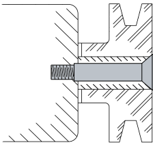
Shoulder Screw as a Shaft
